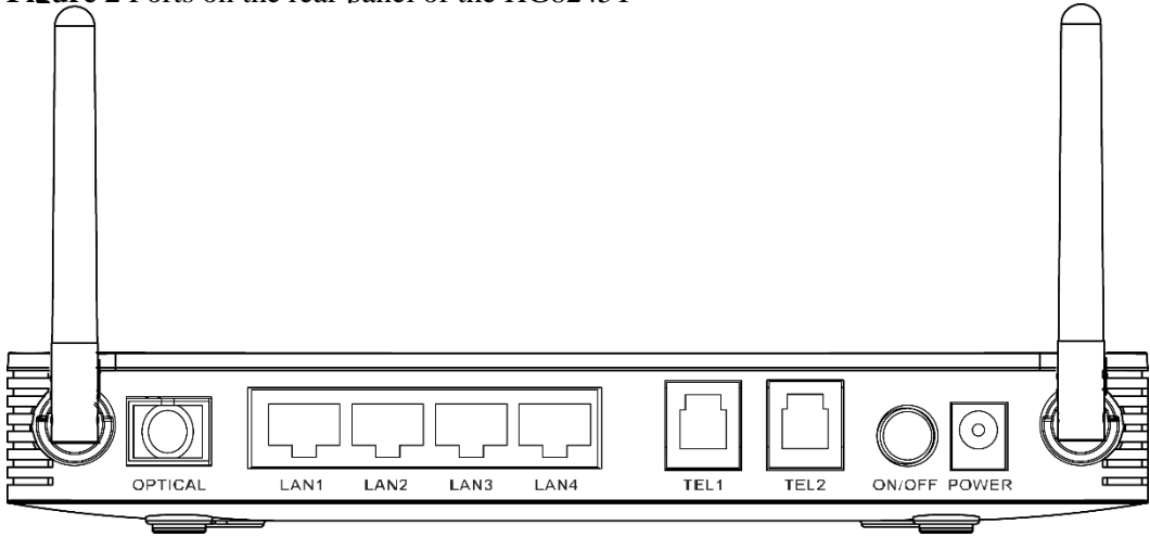
Figure 2 Ports on the rear panel of the HG8245T
