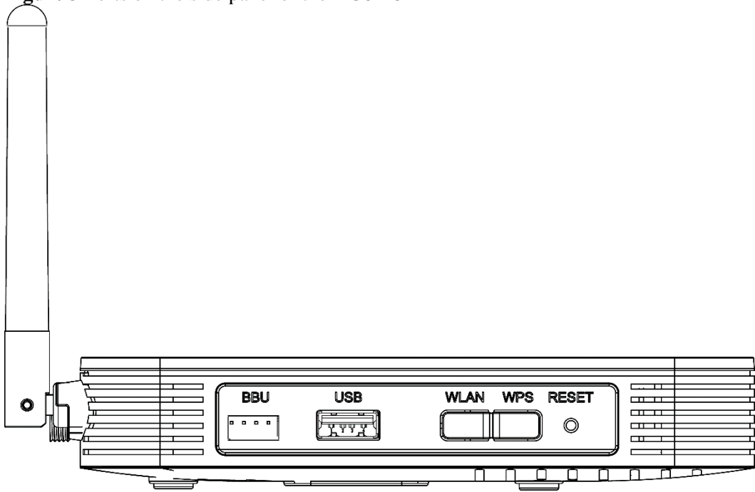
Figure 3 Ports on the side panel of the HG8245T
