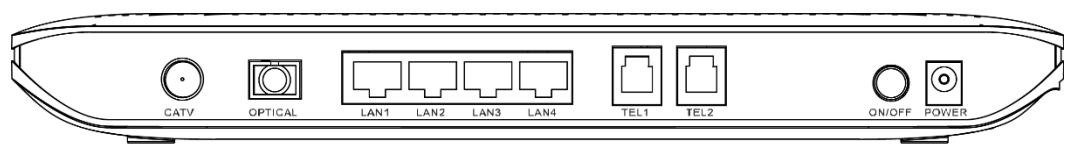
Figure 2 Ports on the rear panel of the HG8242
